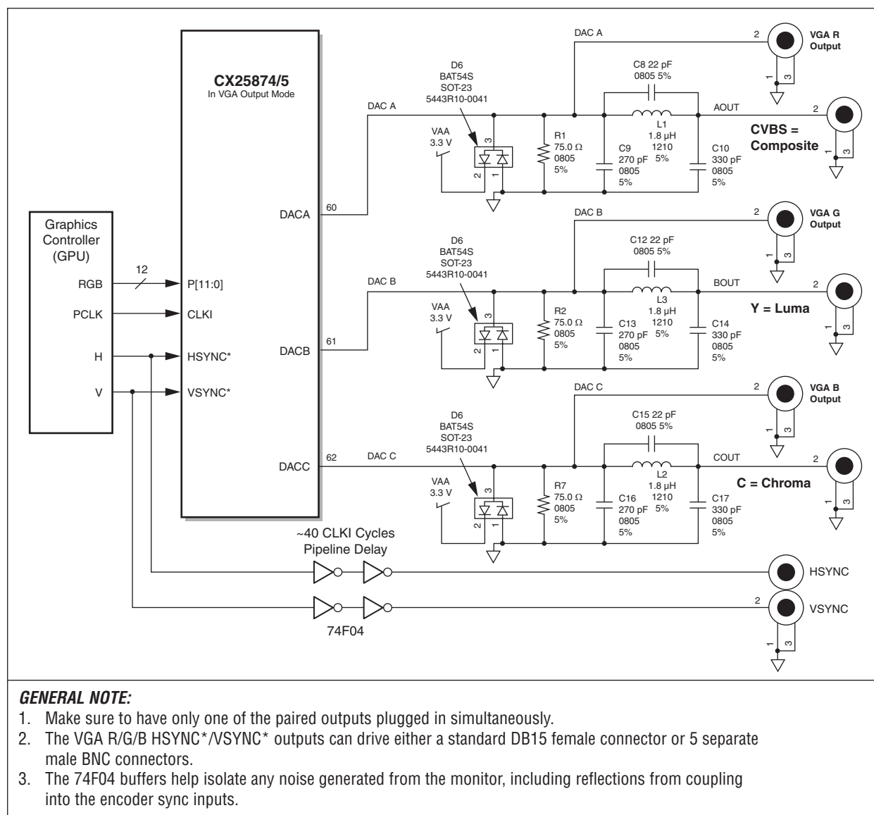
Figure 1-52. Filterless DAC Outputs for VGA (RGB) DAC Output with Sync Buffers
