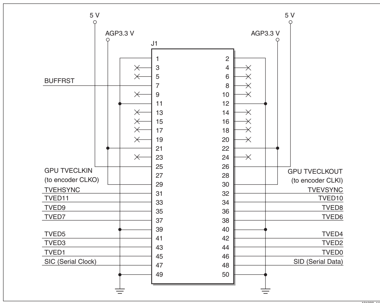
Figure 3-27. Connection Diagram for the Dual-Row 50-pin Header on TV Module / Daughter Card Connection Diagram for the Dual-Row 50-pin Header on Daughter Card/TV Module
