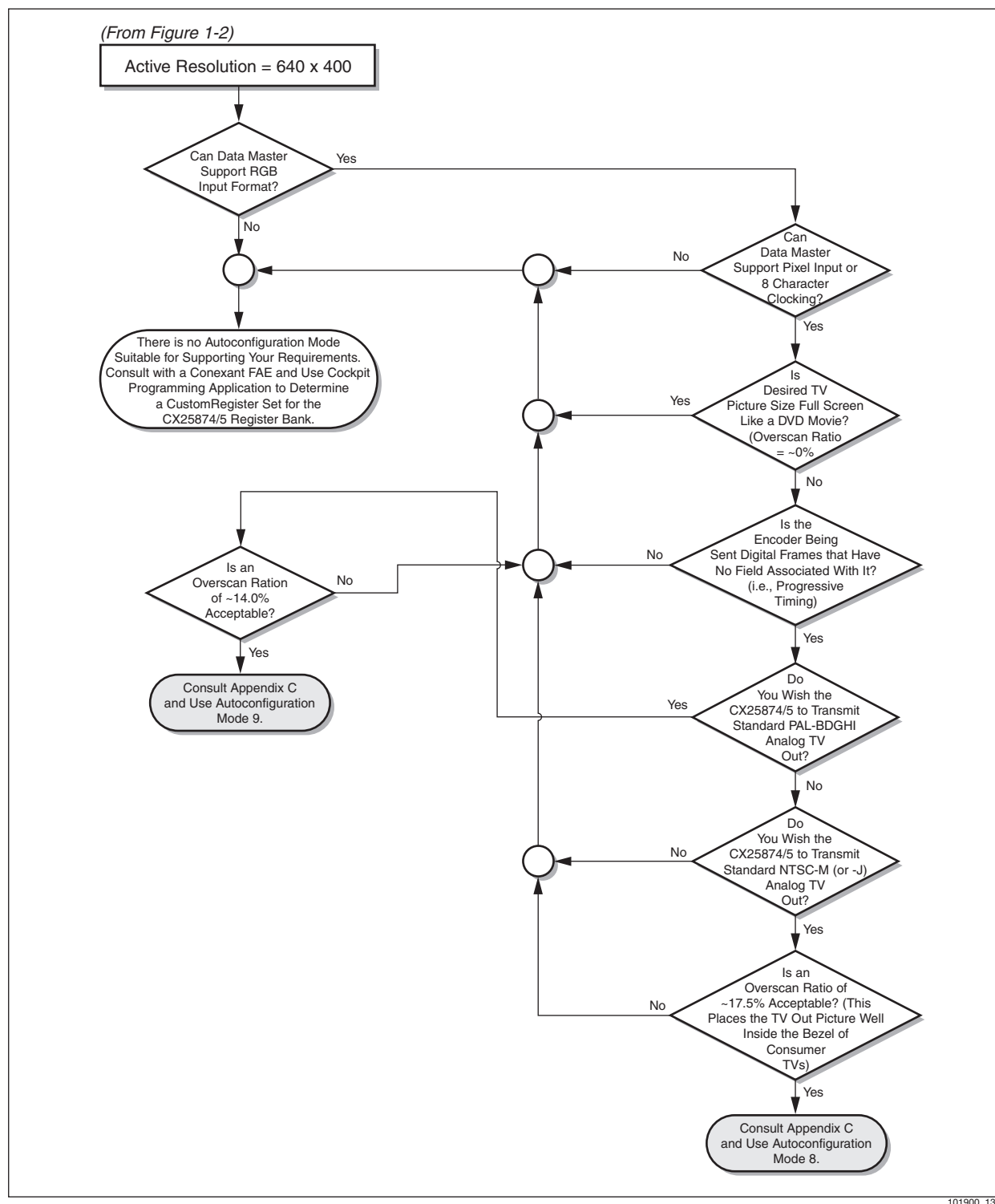
Figure 1-68. Autoconfiguration Mode Programming—640x400
