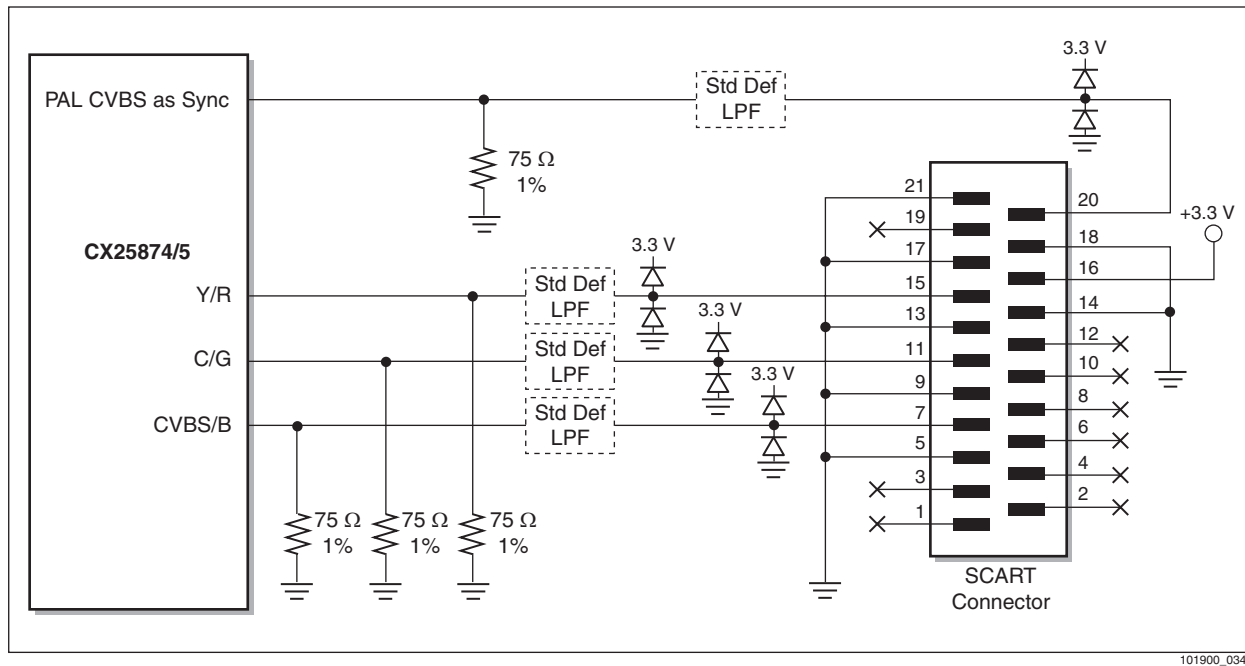
Figure 1-50. CX25874/5 Driving a Type II SCART Connector (Y/C and BBC SCART Compliant)
