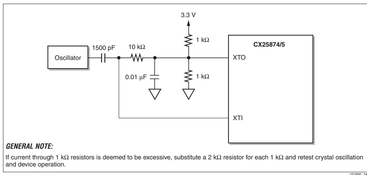
Figure 1-3. Single-Ended Oscillator Biasing Circuit
